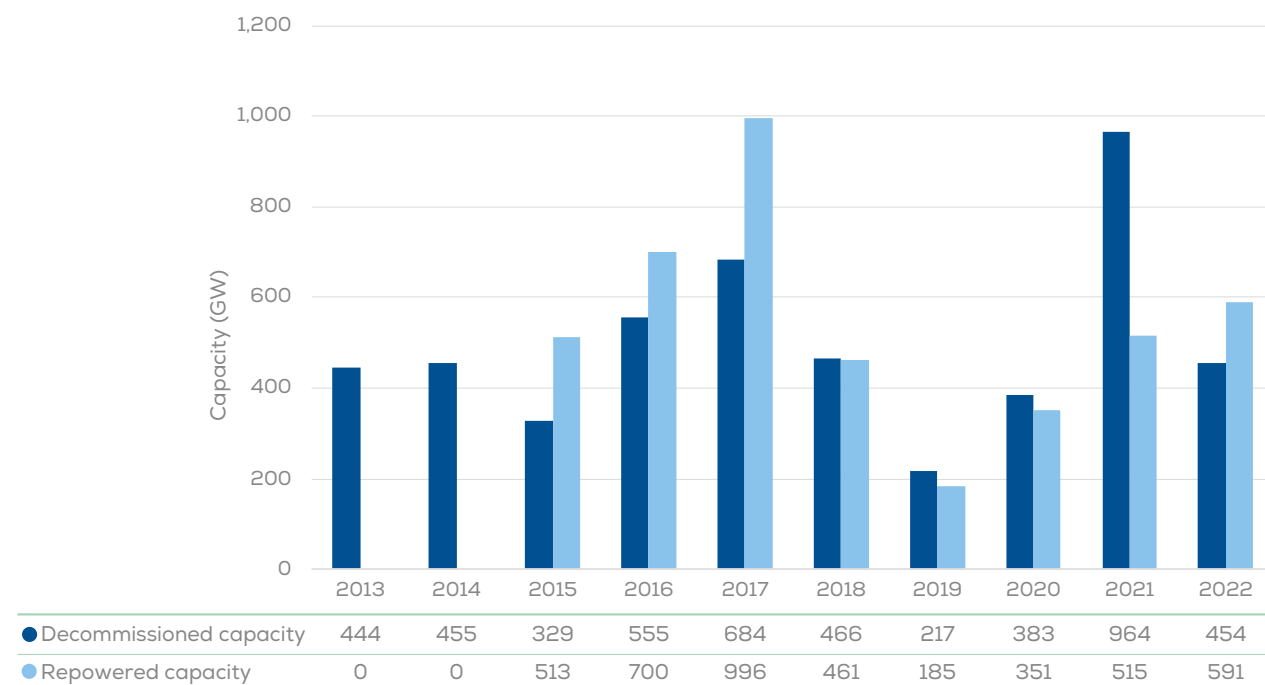
FIGURE 13. Decommissioned and repowered capacity in Europe, 2013-22
